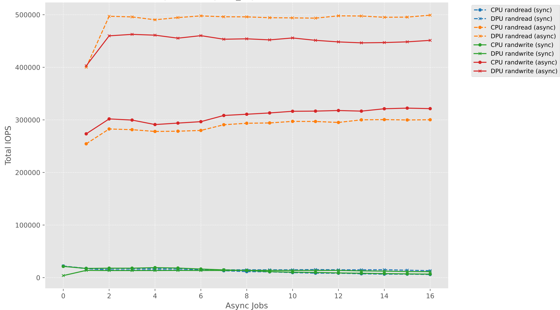
IOPS vs Async Jobs (sync1_asyncN) - RAND (CPU vs DPU)
